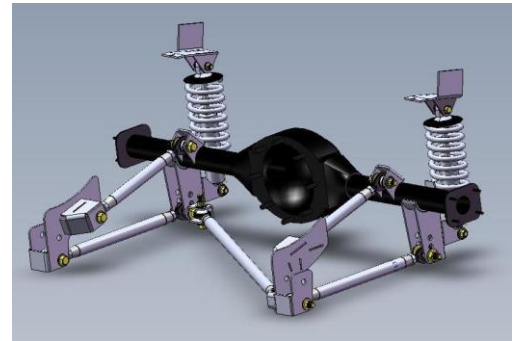
4-Link Coil-Over Rear Suspension Kits AMX, Javelin, Rebel, Ambassador, American, Spirit, Hornet, Gremlin & Concord
